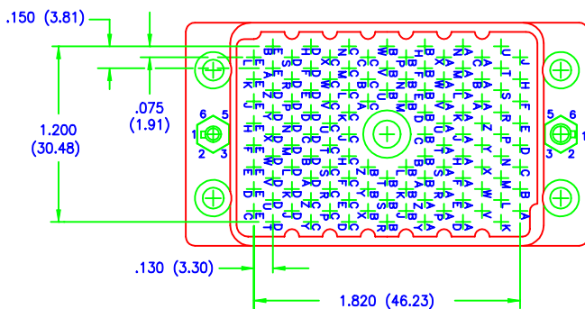
120 PIN PLUG
