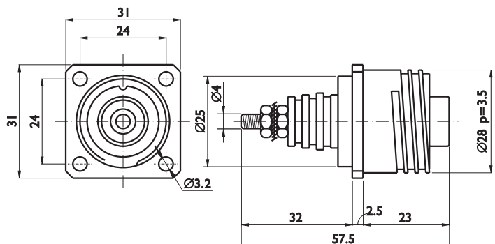
FEMALE RECEPTACLE, AT-21
